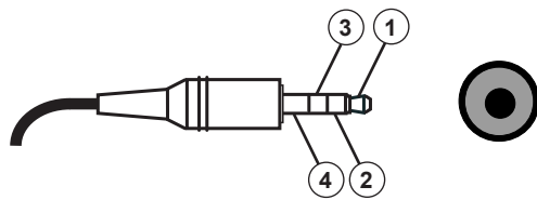
EXTERNAL RS232C CONTROL 3.5 mm Jack on STB
